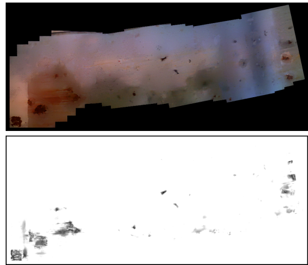
Fig. 8. Visual inspection performance: (top) mosaic built from images collected by the MAV [contrast tuned for visualization purposes], (bottom) defect detection result [darker pixels are likelier to correspond to defects].
