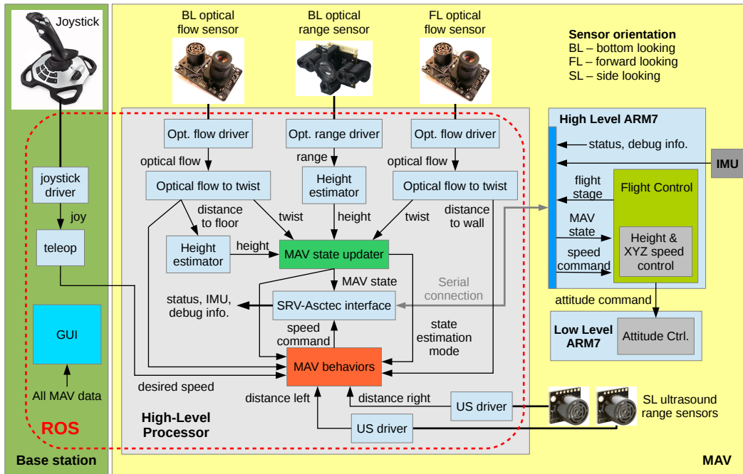
Fig. 2. Full system control architecture.
