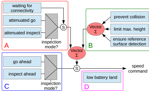
Fig. 3. MAV behaviors: A groups behaviors to accomplish the user intention, B groups behaviors that ensure the platform safety within the environment, C groups behaviors that increase the autonomy level, and D groups behaviors oriented to check flight viability.
