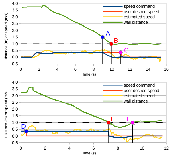
Fig. 6. Performance of some behaviors: (top) the user-desired speed is obeyed ( \rightarrow A), it is attenuated (A \rightarrow B) and cancelled to prevent an imminent collision (B \rightarrow C) until the user-desired speed does become zero (C \rightarrow ); (bottom) the user-desired speed is sustained while the wall is at enough distance (D \rightarrow E), it is cancelled and even forced to be negative to prevent an imminent collision (E \rightarrow F) until the platform is again at the safe distance (F \rightarrow ). All units are in SI (m or m/s accordingly).
