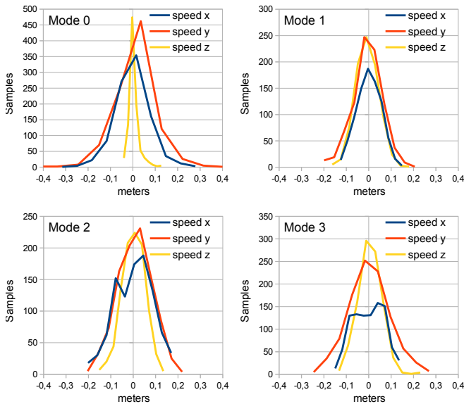
Fig. 5. Histograms of estimated speeds for 1-minute hovering flights for the four state estimation modes.
