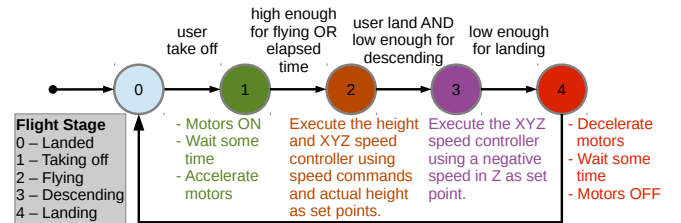
Fig. 4. Flight control state machine.
