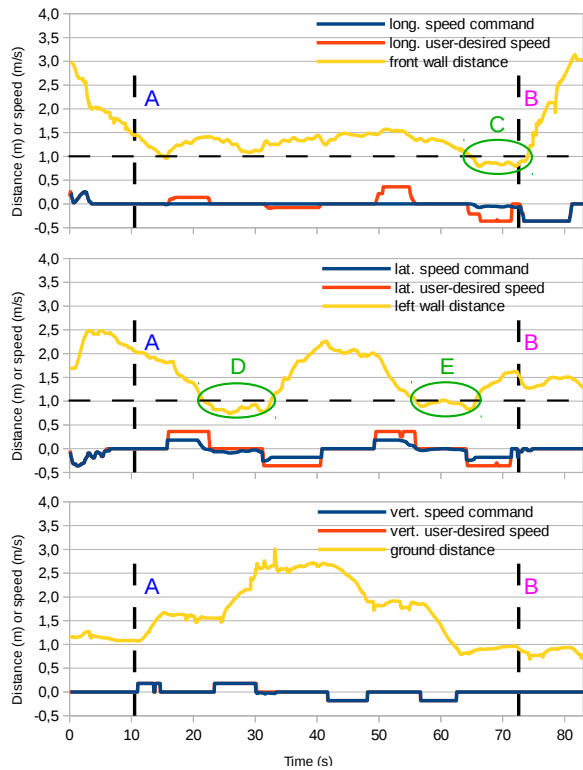
Fig. 7. Performance of the platform during an inspection task using the inspection mode (A→B). All units are in SI (m or m/s accordingly).
